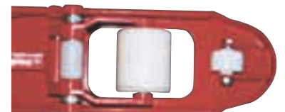
Two nylon entry and exit rollers (wide models only)
