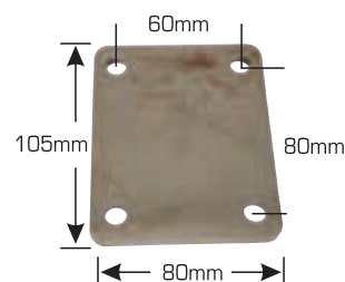
MC-Plate Weld on mounting plate for 'MC' series castors
